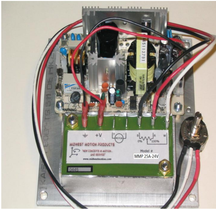
Integrated AC / DC Power Supply and Motor Speed Control mounted to a 6" Square Chassis.
